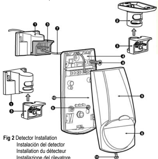
Fig 2 Detector Installation
